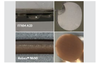
High Temperature PECVD process: FFKM A33 vs. Kalrez® 9600
